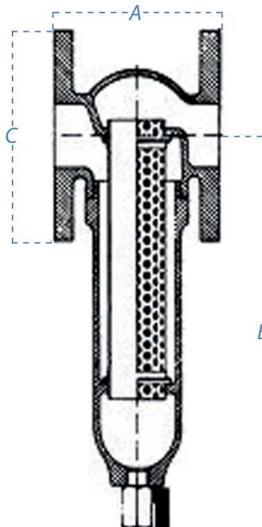
Type RF Flenset
